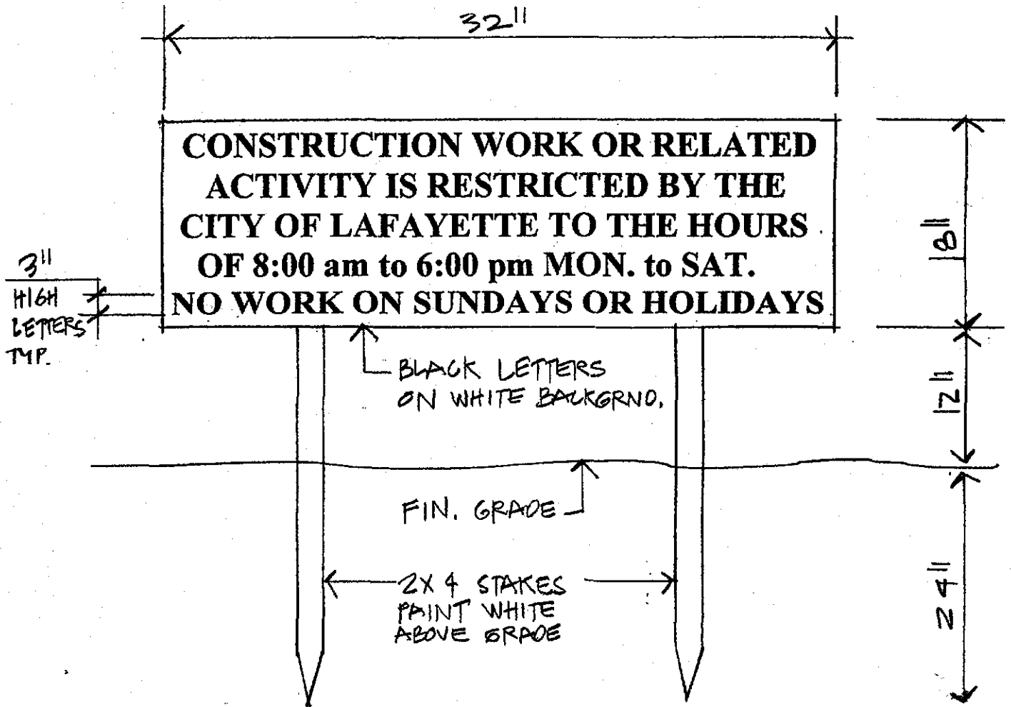
1 CONSTRUCTION HOURS SIGN DETAIL
